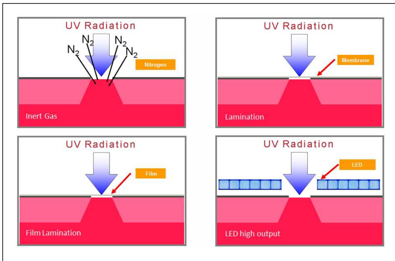
Figure 2: Flat top dot solutions available to date in the market.
